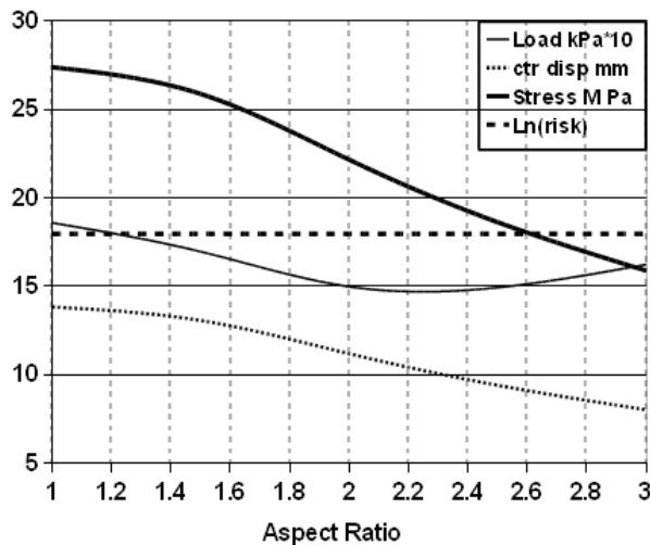
Figure 3: Design (8/1000) capacity, kPa; centre displacement, mm; maximum stress, MPa; and Ln(risk function) for a glass plate of thickness 5.66 mm and area 2 m 2 , plotted against aspect ratio (height/width).
