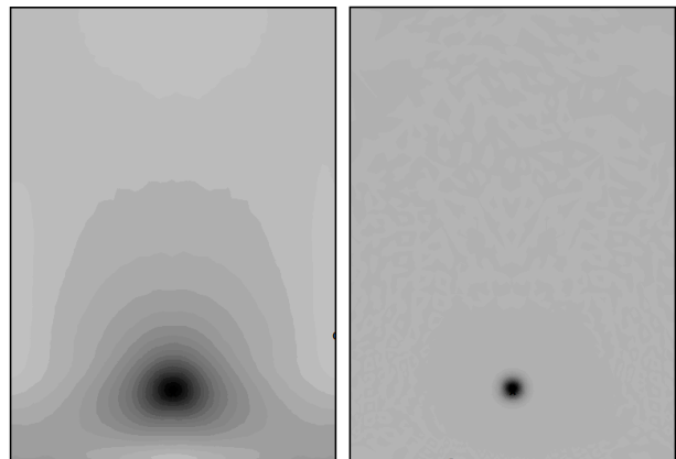
Figure 4: Stress and Risk density distributions for 1.5 kN point load (governing load for the glass guard in this case).
